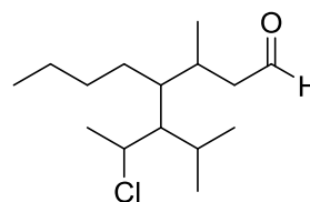
4-(2-chloro-4-methylpentan-3-yl)-3-methyloctanal
