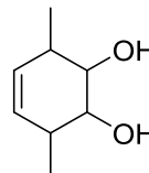
3,6-dimethylcyclohex-4-ene-1,2-diol
