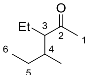
3-ethyl-4-methylhex-2-one
