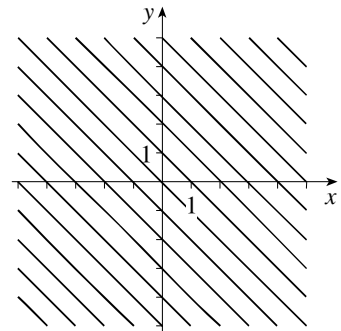
\sin(\pi(x+y)) = 0
