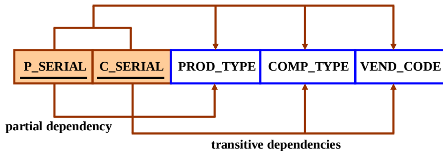
The Original Dependency Diagram
