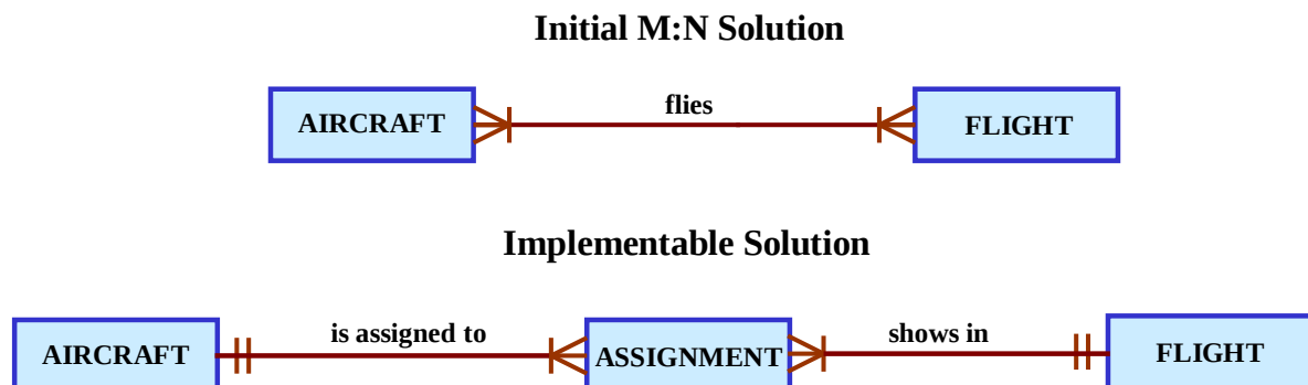
FIGURE P2.16c The Airline Crow's Foot ERD
