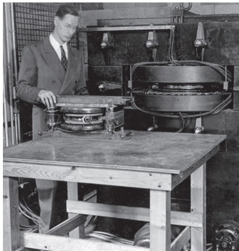
FIGURE 2.4. A Betatron accelerates particles using the electric field from magnetic induction. The diagram shows the principle, and defines quantities that allow us to derive the so-called Betatron Condition . The photograph (Courtesy Department of Physics, University of Illinois at Urbana-Champaign) shows early Betatrons with inventor, Donald Kerst.
